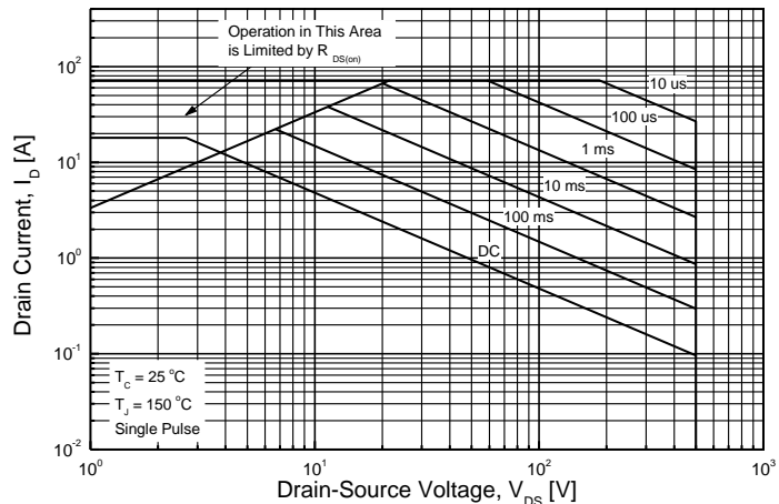
TMPF20N50A(G)
